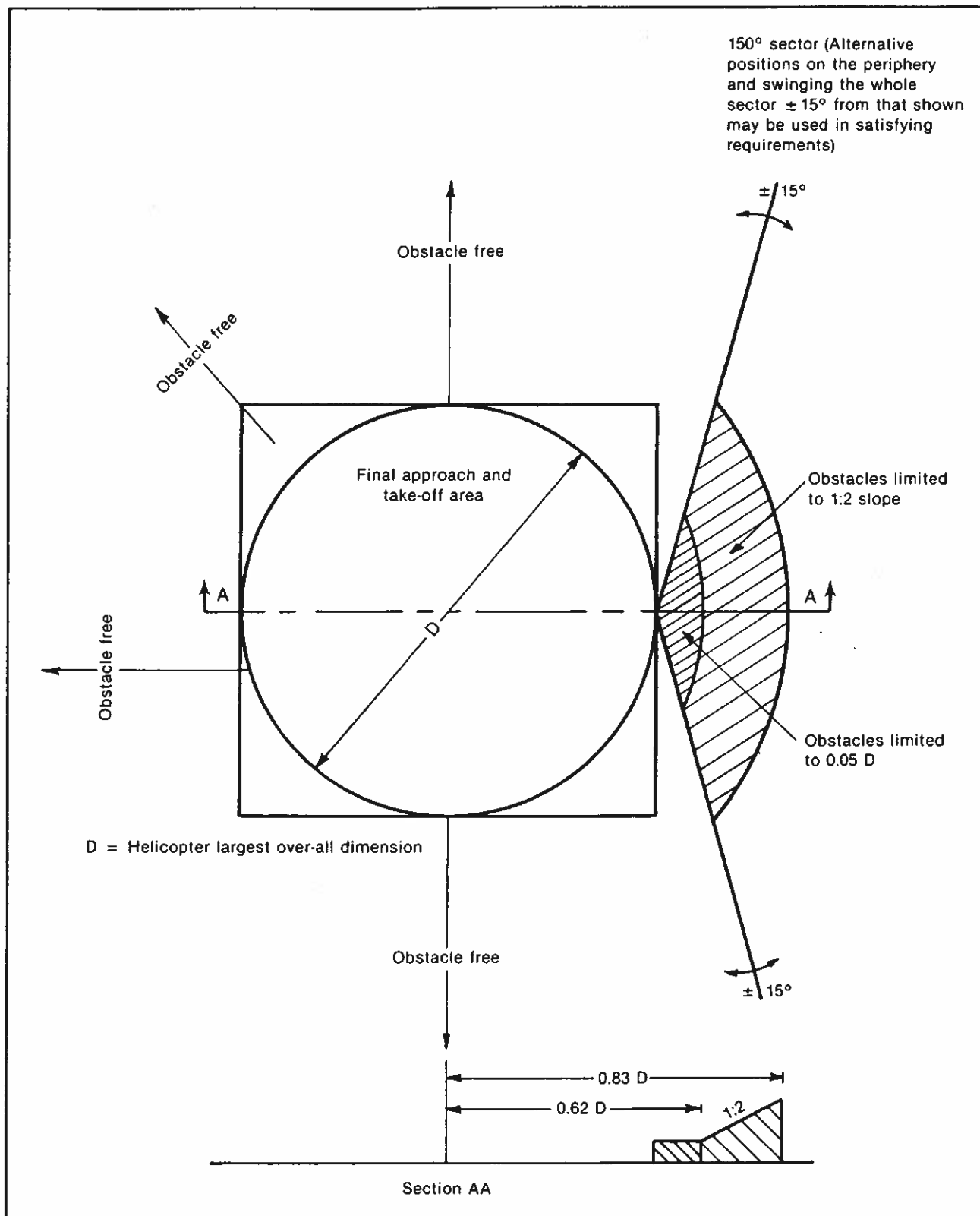
Figure 3-4. Helideck obstacle limitation sectors Single-main-rotor and side-by-side twin rotor helicopters
