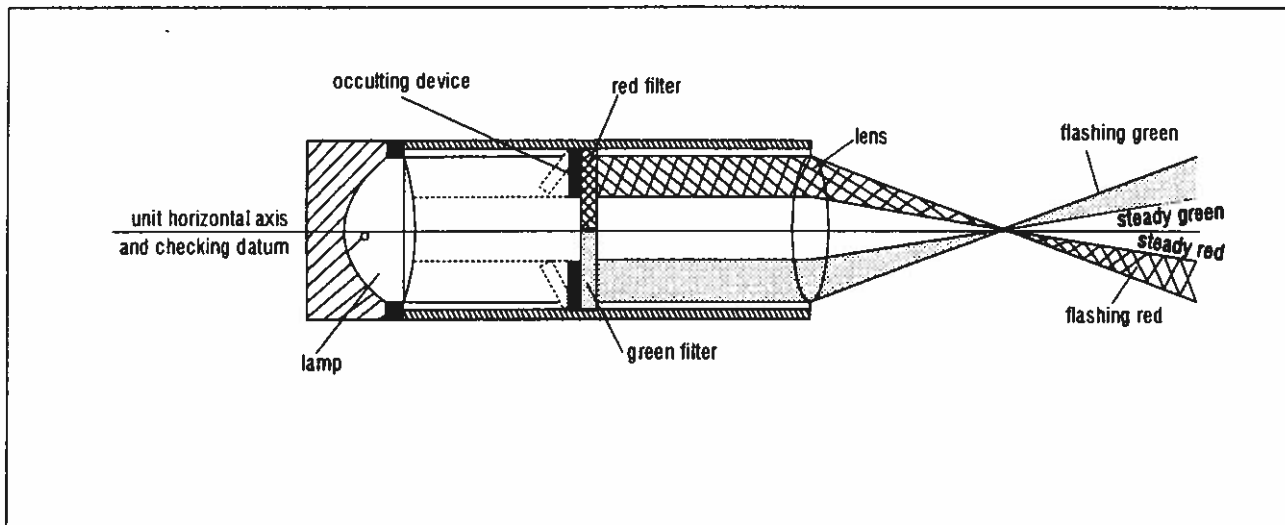
Figure 5-17. HAPI light unit
