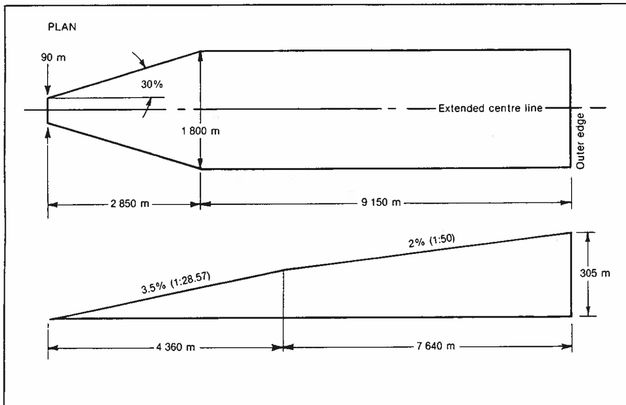
Figure 3-10. Take-off climb surface for instrument FATO
