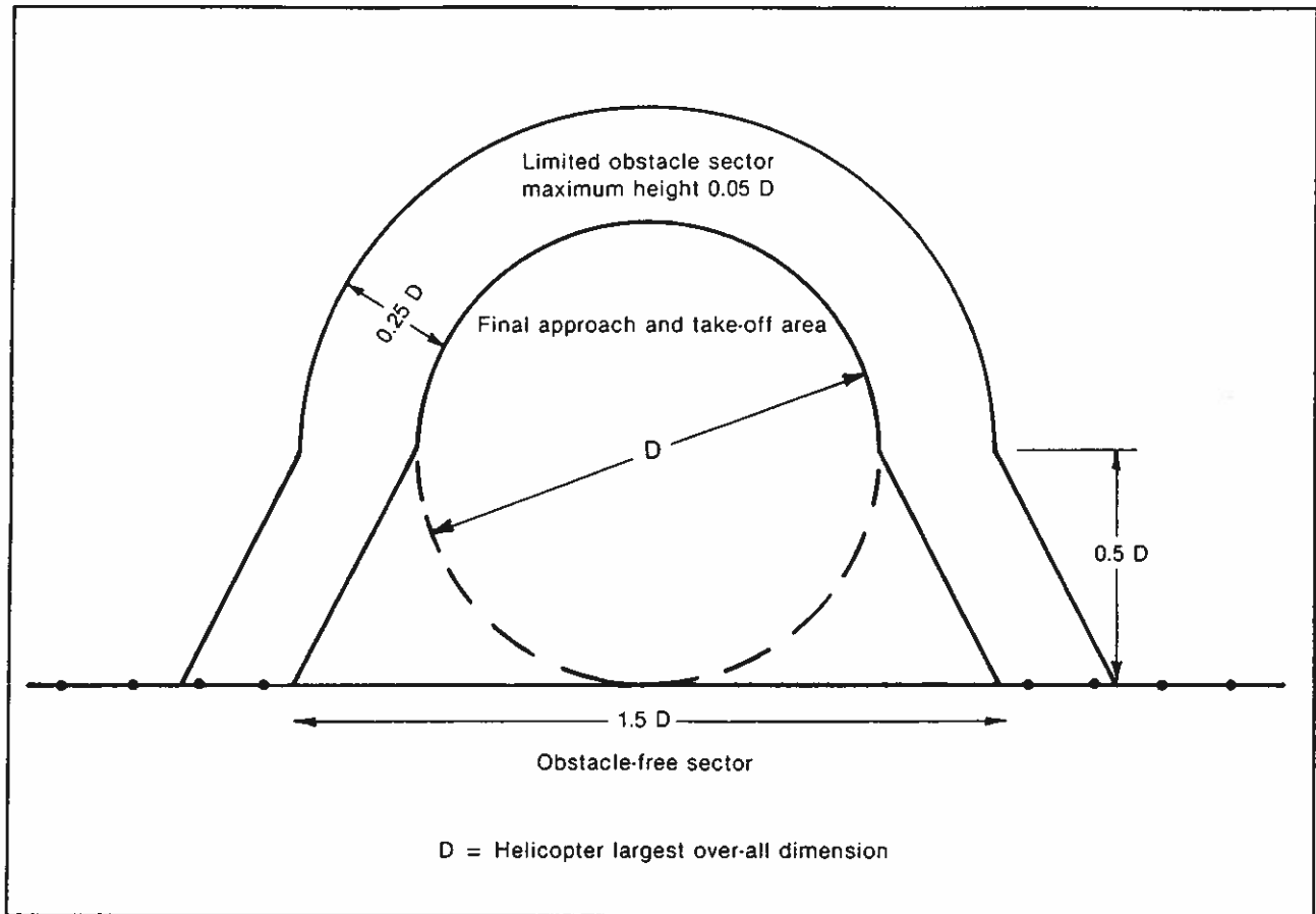
Figure 3-15. Ships-side non-purpose built heliport obstacle limitation surfaces
