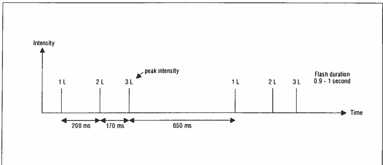
Figure 5-16. Offset sector flash characteristics
