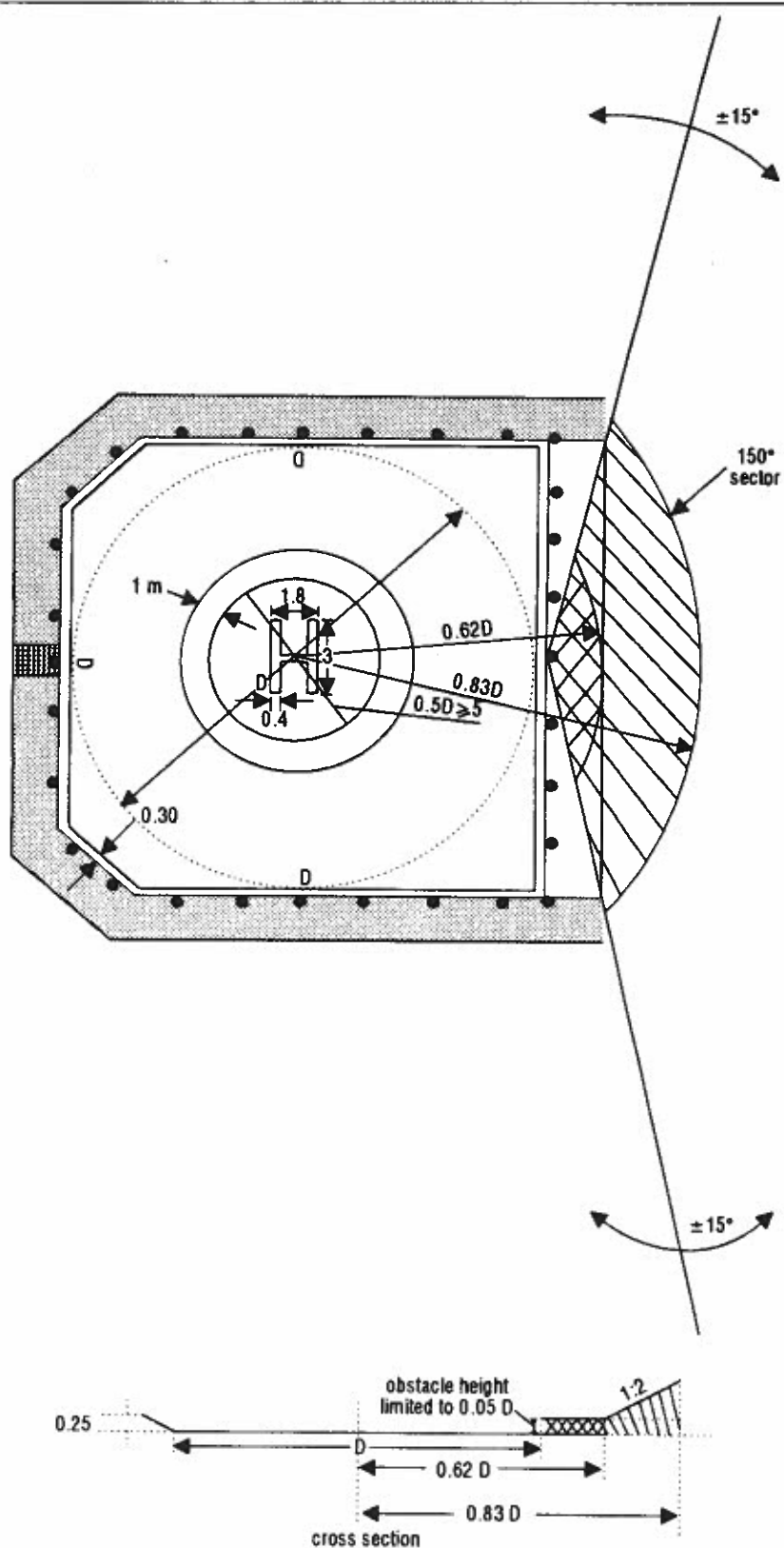
Figure 5-13. Location of touchdown marking Example A. Centred touchdown marking
