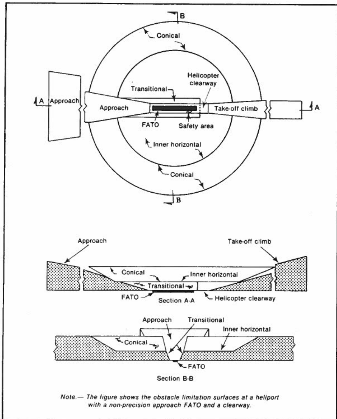
Figure 3-1. Obstacle limitation surfaces
