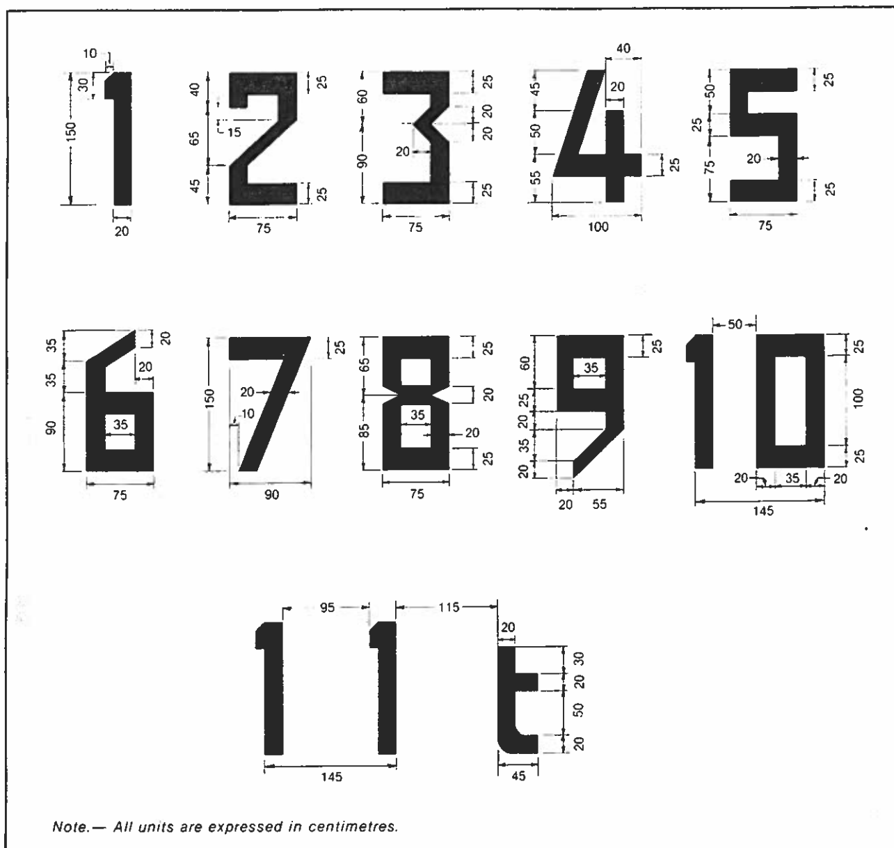
Figure 5-12. Form and proportions of numbers and letter for maximum allowable mass marking
