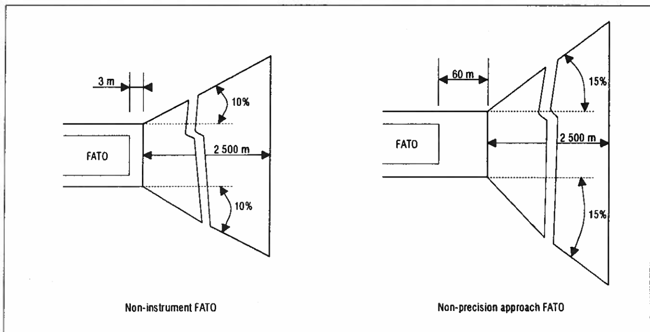
Figure 5-19. Area to be surveyed
