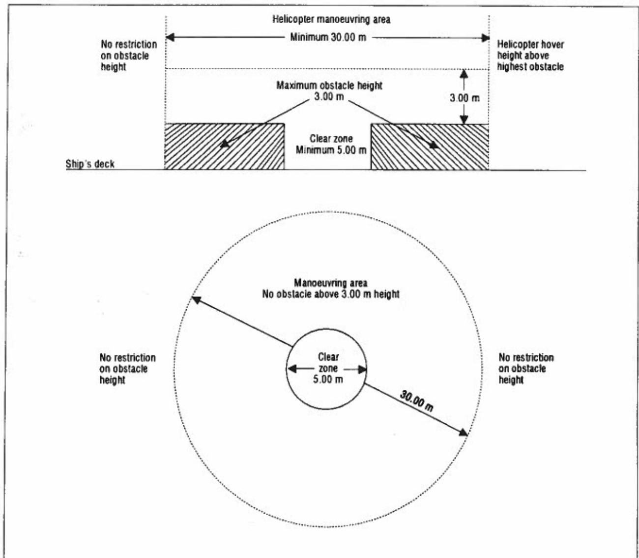
Figure 4-1. Winching area
