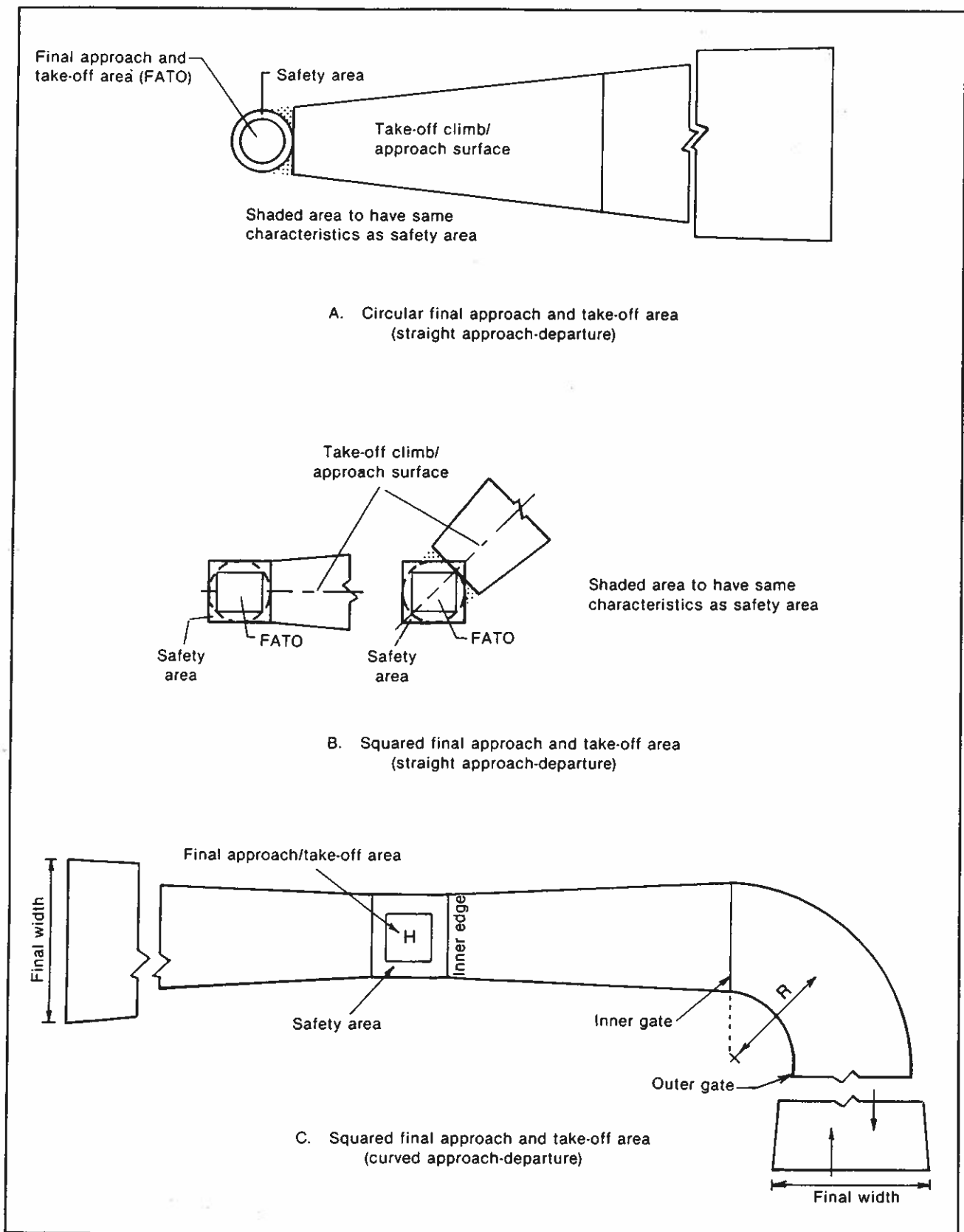
Figure 3-7. Take-off climb/approach surface (non-instrument FATO)
