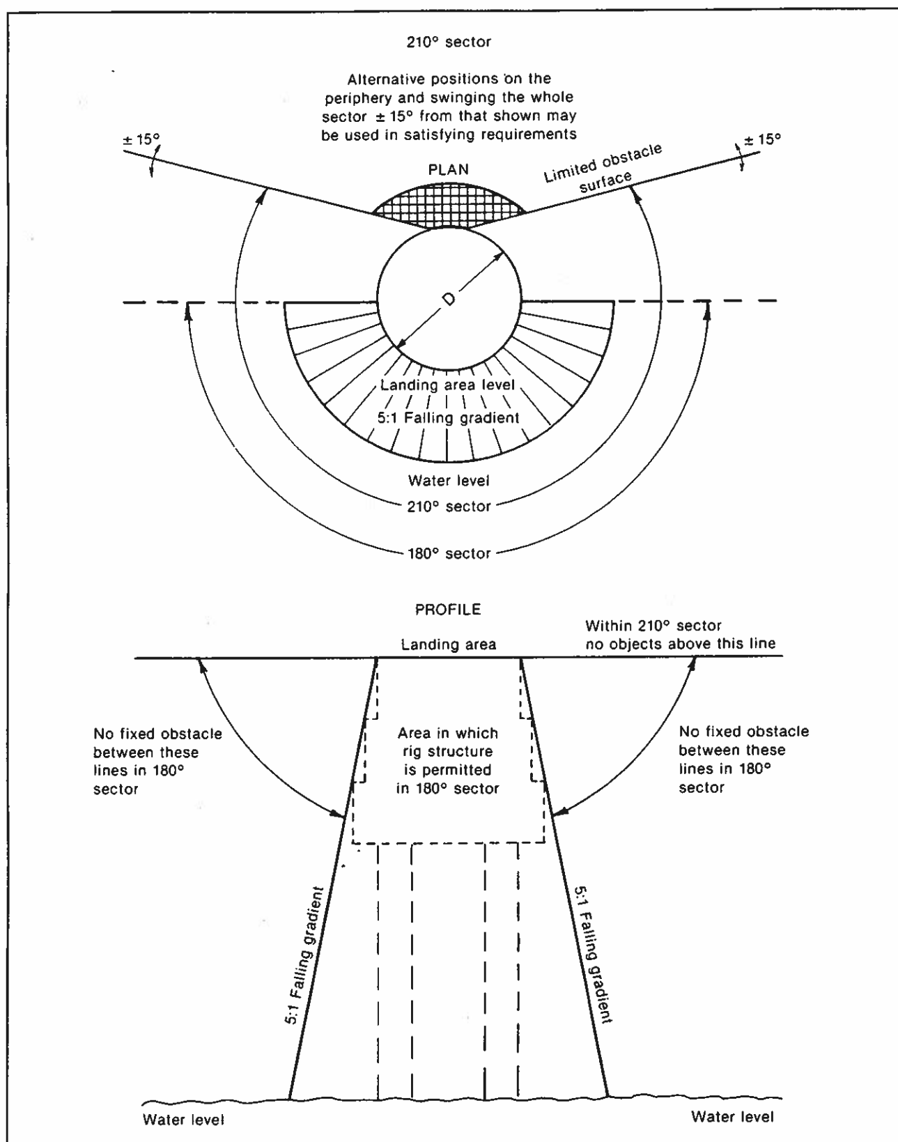
Figure 3-2. Helideck obstacle-free sector
