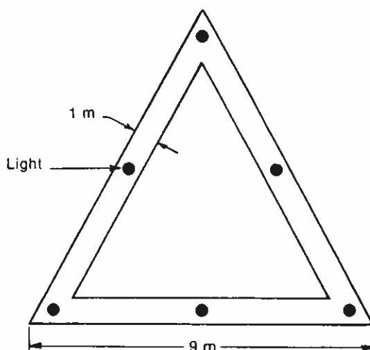
Figure 5-5. Aiming point marking and lighting
