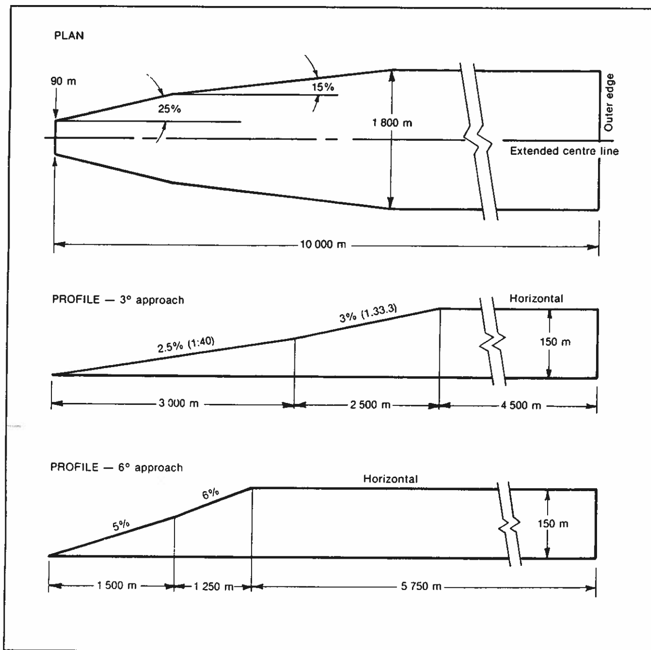
Figure 3-11. Approach surface for precision approach FATO
