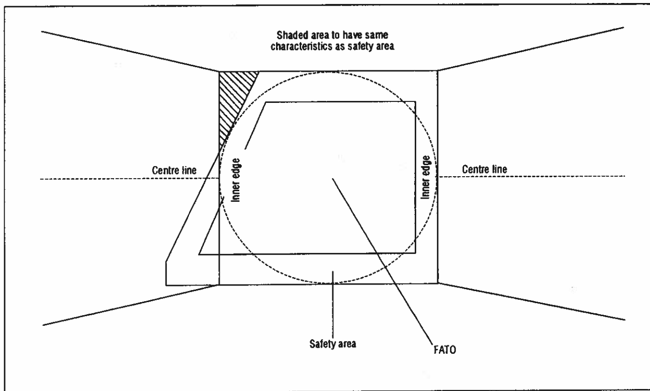
Figure 3-8. Take-off climb/approach surfaces (irregular shaped non-instrument FATO)
