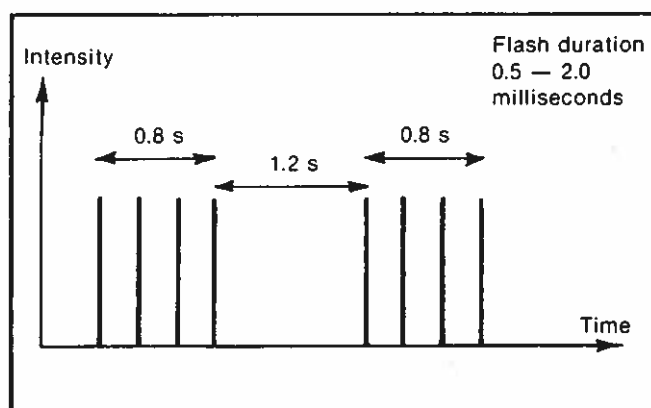
Figure 5-9. Heliport beacon flash characteristics
