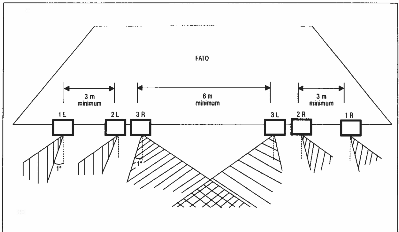
Figure 5-15. Siting of the alignment guidance system
