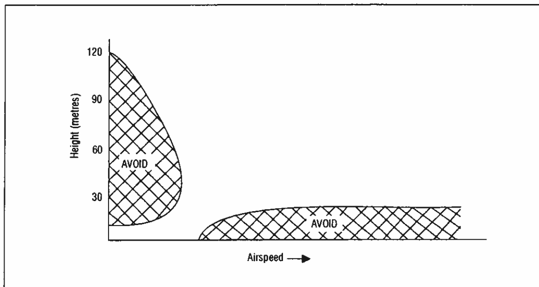
Figure 1-1 Typical combinations of height and airspeed to be avoided
