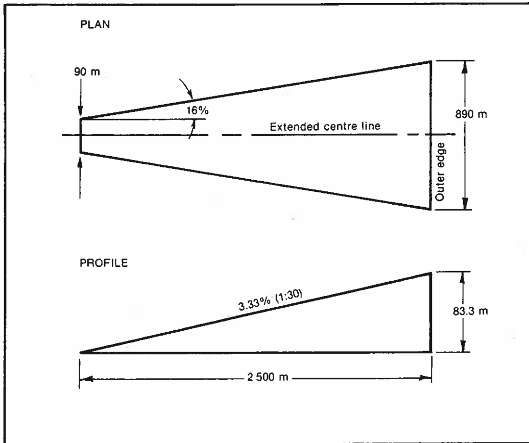
Figure 3-12. Approach surface for non-precision approach FATO
