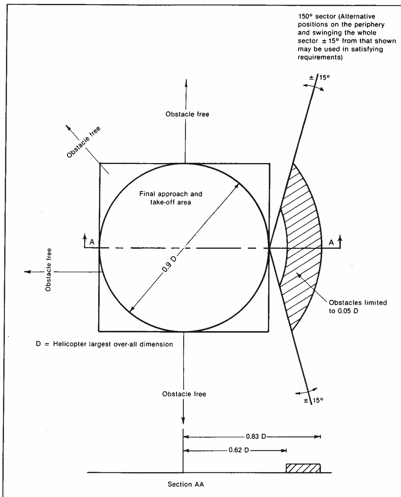
Figure 3-5. Helideck obstacle limitation sectors Tandem-main-rotor helicopters — Omnidirectional operations
