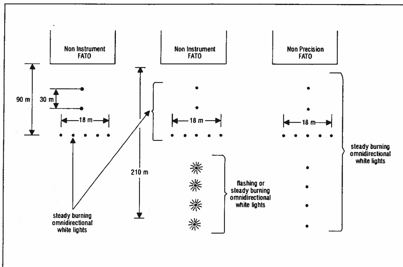
Figure 5-10. Three different configurations of an approach lighting system
