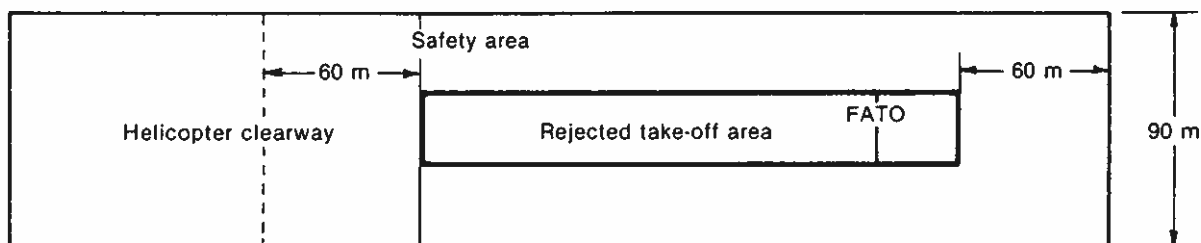
Figure 2-1. Safety area for instrument FATO
