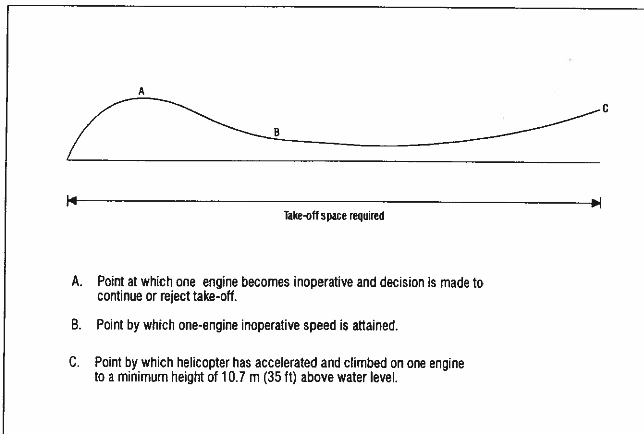
Figure 3-3. Take-off space required
