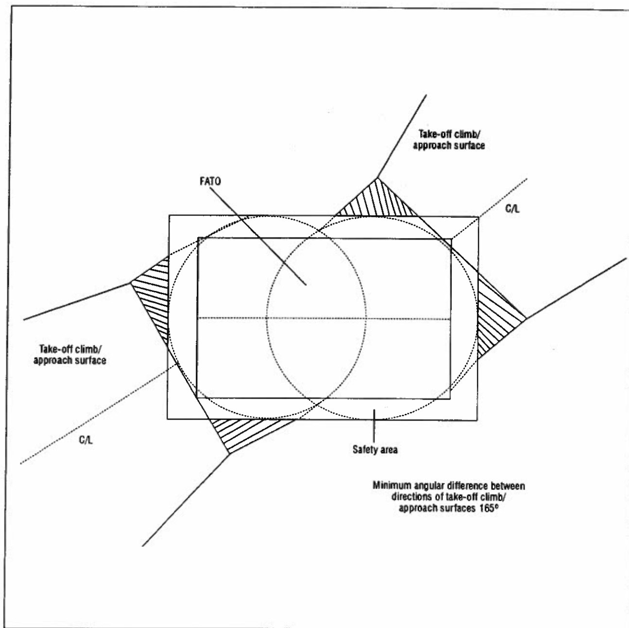
Figure 3-9. Take-off climb/approach surfaces (larger than minimum specified non-instrument FATO)
